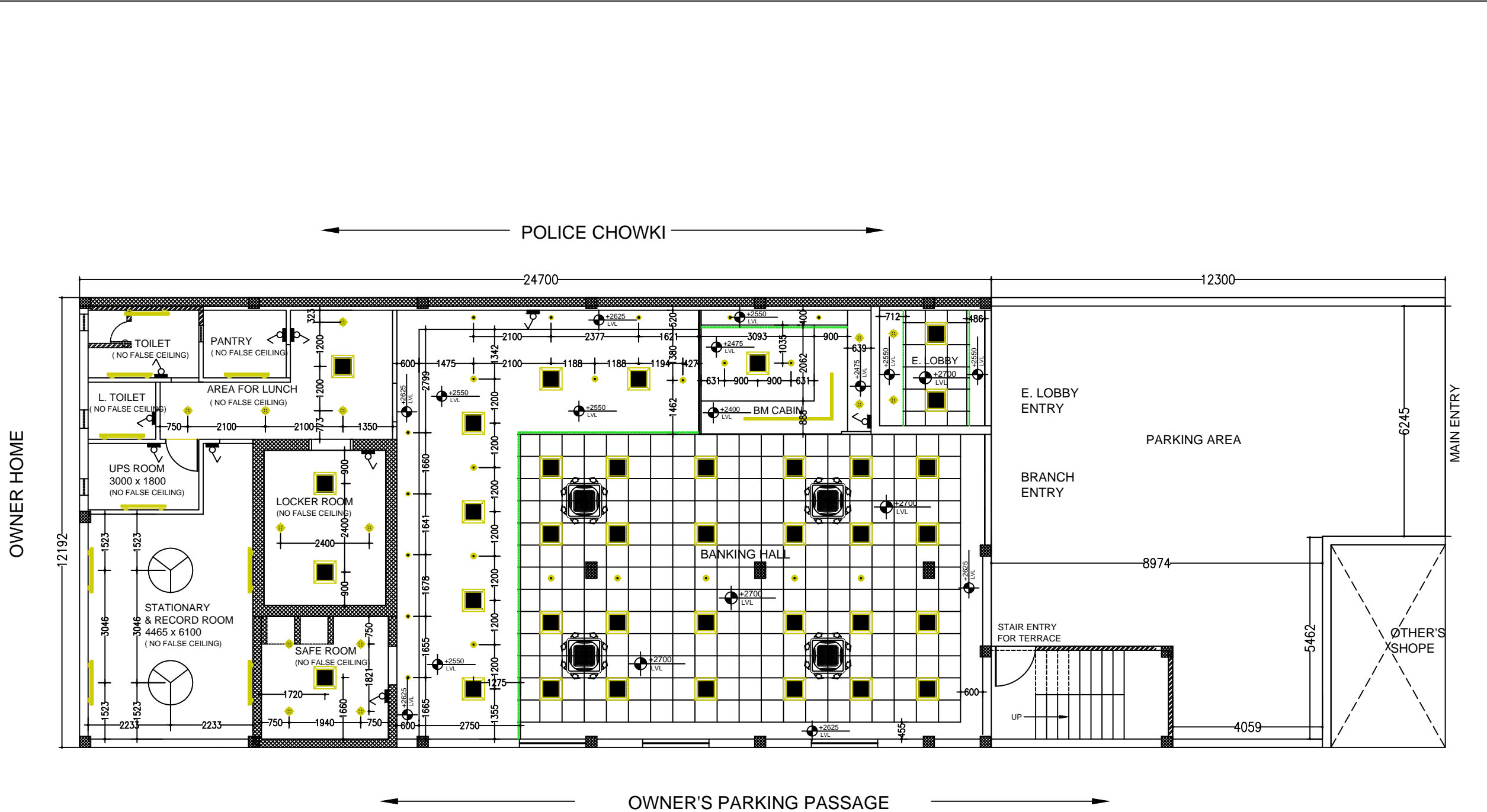
GROUND FLOOR LAYOUT PLAN
